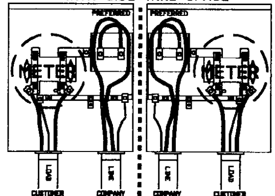
200 AMP UNDERGROUND METERBASE WITH SIDE WIRE SPACE
